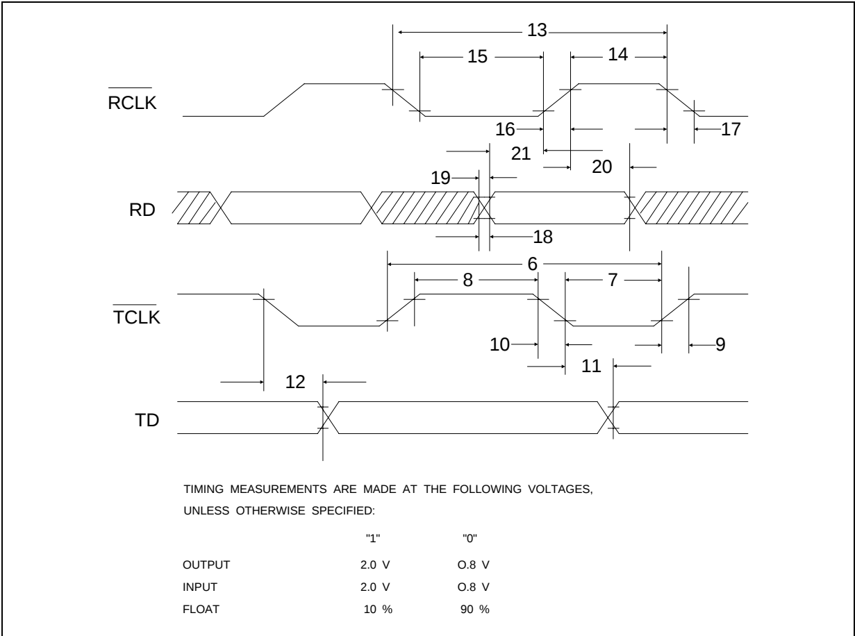
Figure 6: MK50H25 Serial Link Timing Diagram
