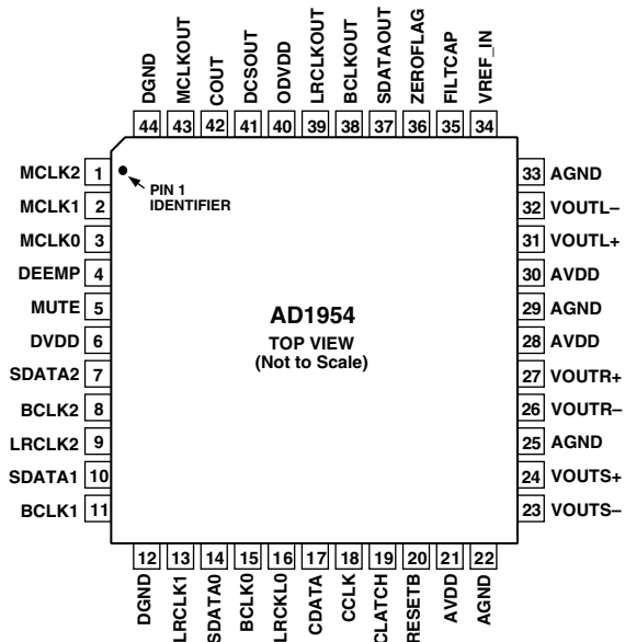
44-Lead MQFP
