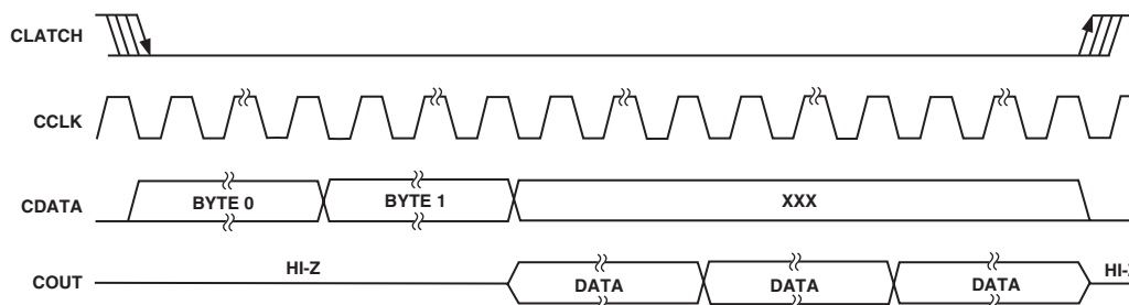
Figure 16. Sample of SPI READ Format (Single-Read Mode)
