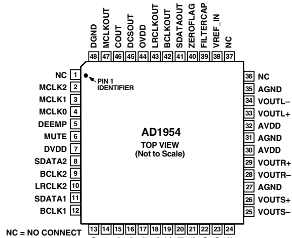
48-Lead LQFP
