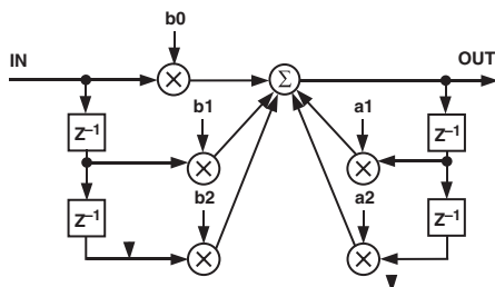
Figure 4. Biquad Filter
