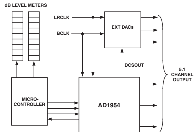
Figure 18. Typical Application of Data Capture Feature
