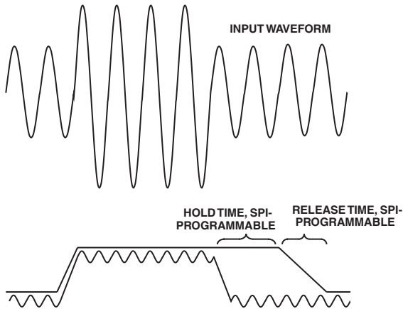
Figure 8. Using the Hold and Release Time Feature
