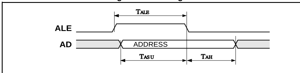
Figure 5: ALE Signal
