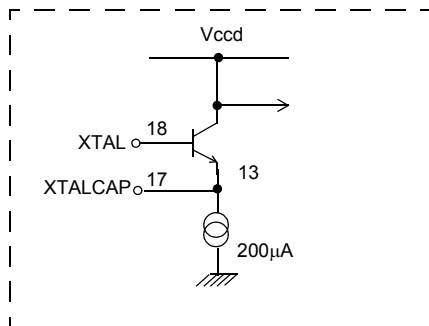
Reference oscillator
