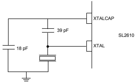
Figure 6 - Crystal Oscillator Application
