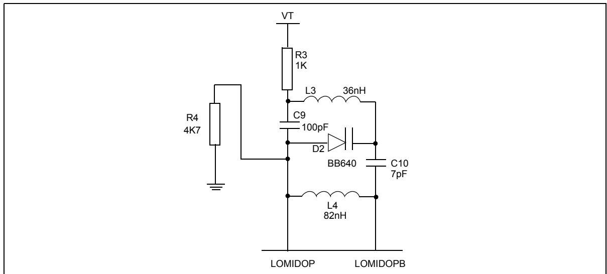
Figure 9 - Mid Band VCO Application
