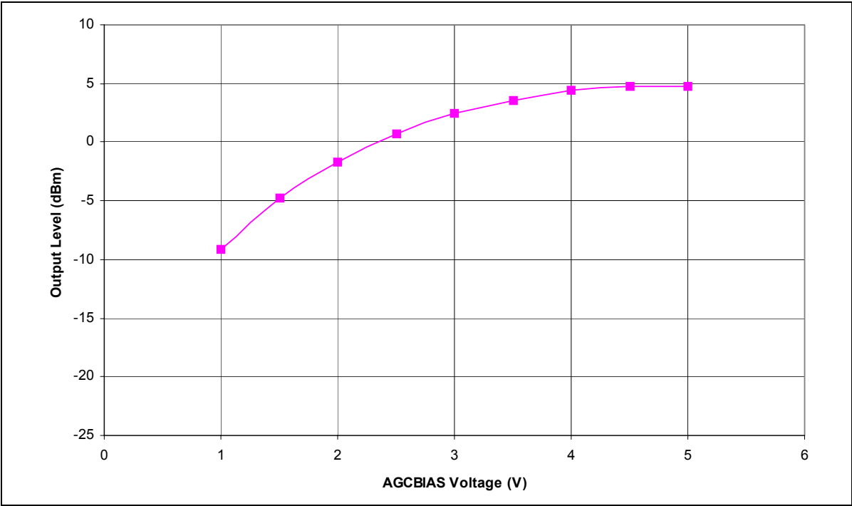
Figure 18 - Typical AGC Output Level Set versus AGCBIAS Voltage
