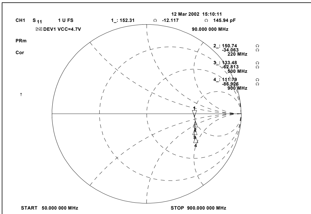
Figure 11 - LO, MID and HI Band Input Impedance
