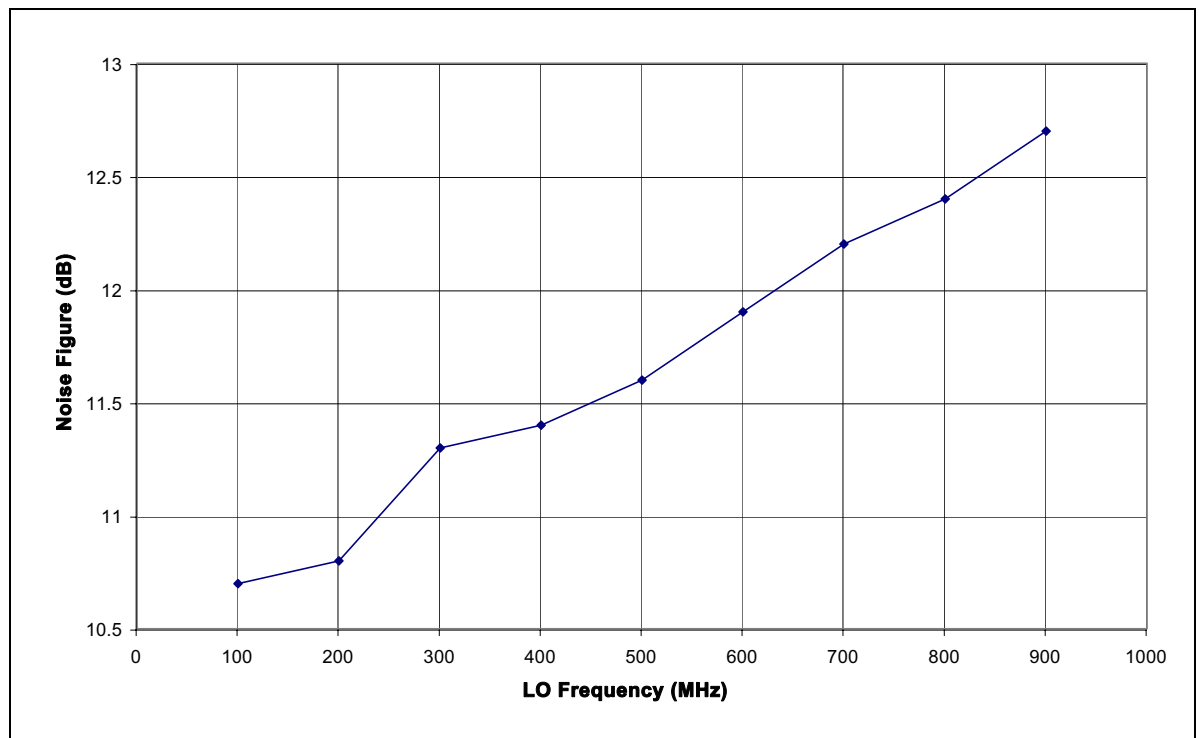
Figure 12 - Low, Mid and Hi Band Noise Figure versus Frequency
