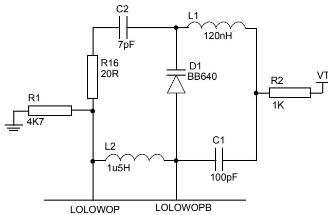
Figure 8 - LO Band VCO Application
