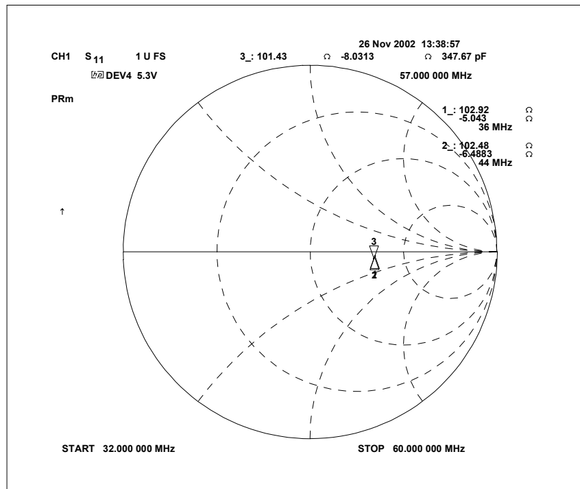
Figure 15 - Converter Output Impedance (Single Ended)
