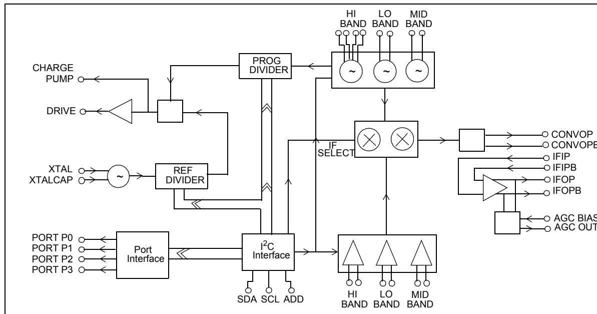
Figure 2 - SL2610 Block Diagram
