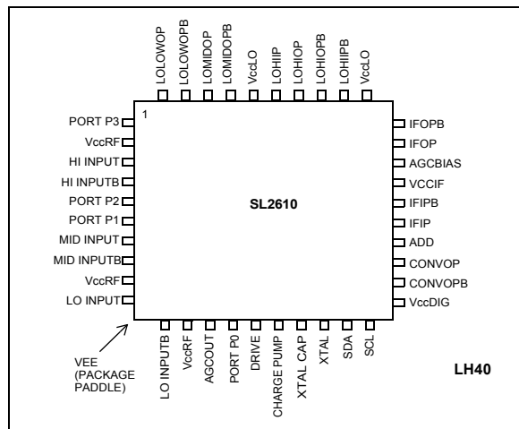
Figure 1 - Pin Allocation Diagram
