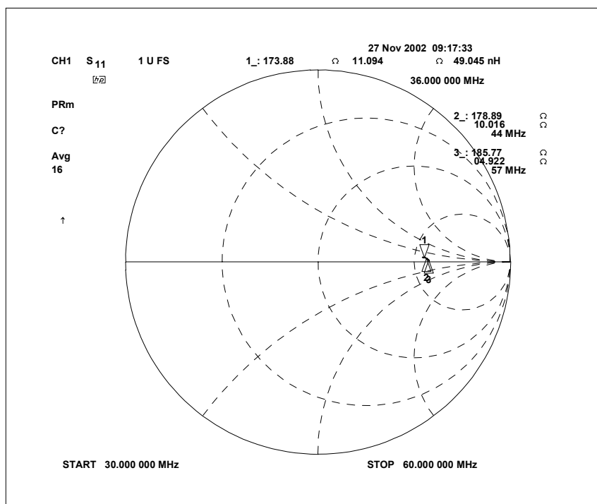
Figure 16 - IFAMP Input Impedance
