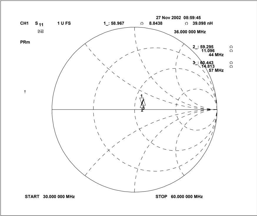
Figure 17 - IFAMP Output Impedance (Single Ended)
