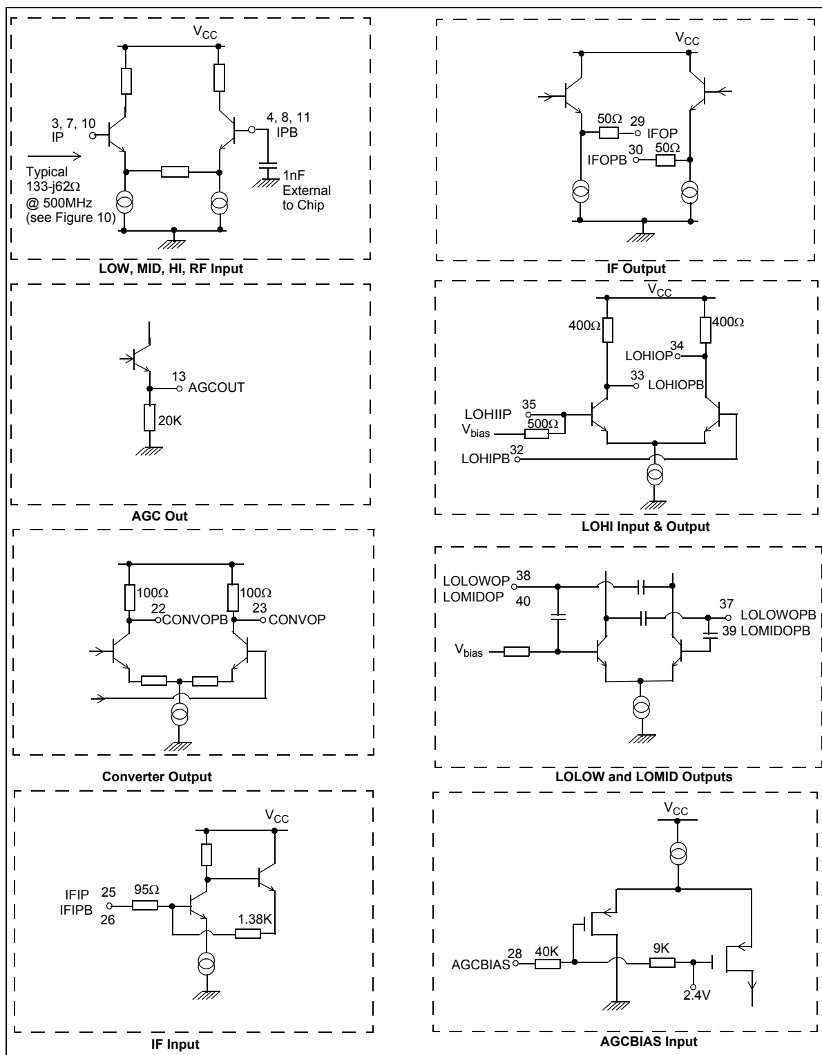
Figure 19 - Input and Output Interface Circuits (RF section)
