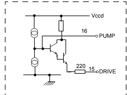
Loop amplifier
