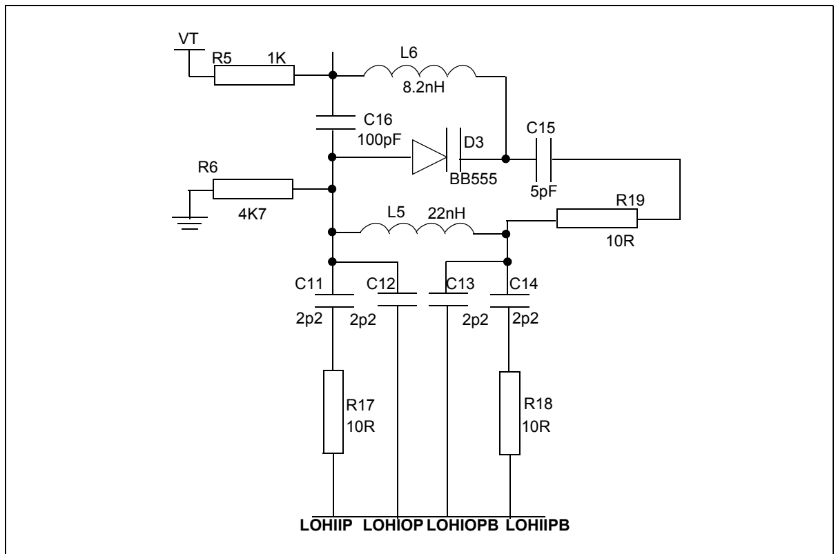
Figure 10 - HI Band VCO Application
