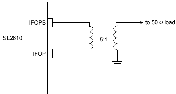
Figure 7 - Ifamp Output Load Condition for Test Purposes
