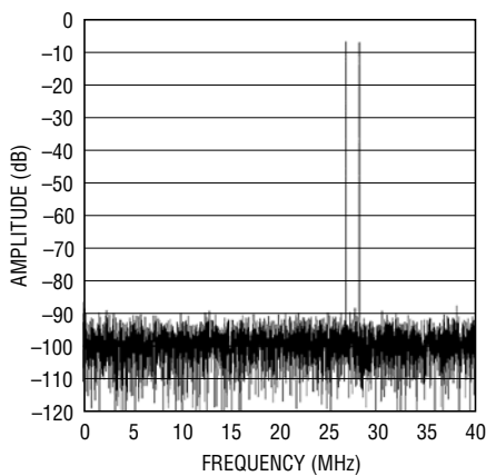
8192 Point 2-Tone FFT, f_{IN} = 28.2\text{MHz} and 26.8\text{MHz} , -1\text{dB} , 2V Range
