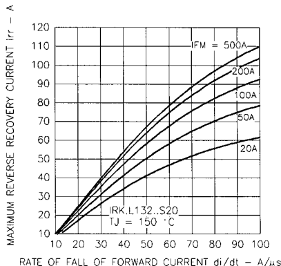
Fig. 12 - Reverse Recovery Current Characteristics
