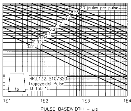
Fig. 13 - Maximum Forward Energy Power Loss Characteristics
