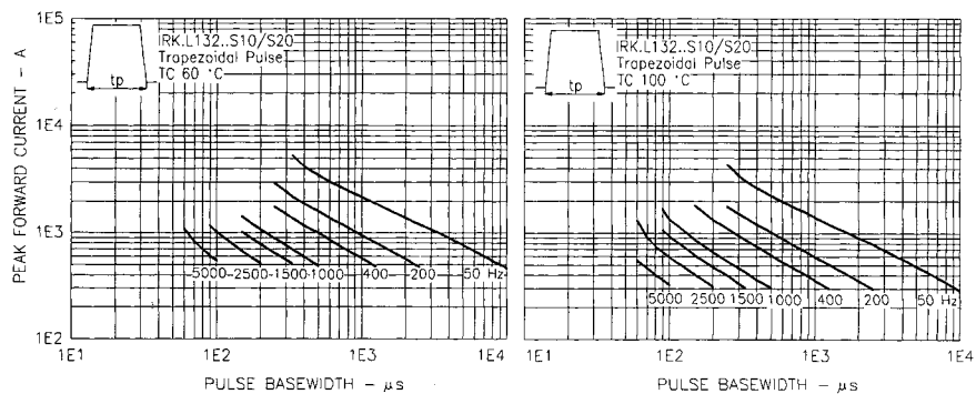
Fig. 15- Frequency Characteristics
