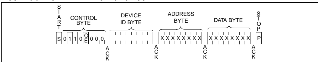
FIGURE 6-3: SET WRITE PROTECTION COMMAND
