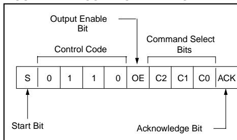
FIGURE 4-1: CONTROL BYTE FORMAT
