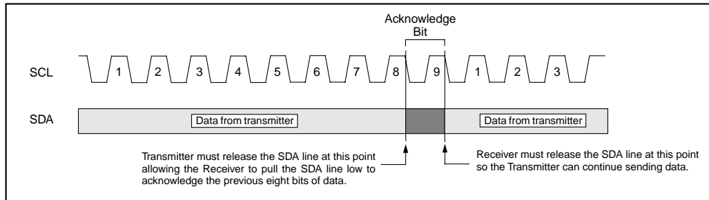
FIGURE 3-2: ACKNOWLEDGE TIMING
