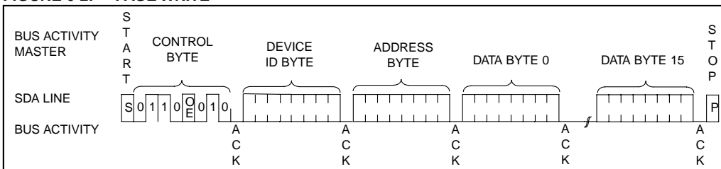
FIGURE 6-2: PAGE WRITE
