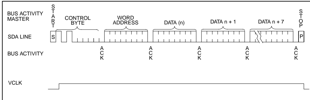
FIGURE 5-2: PAGE WRITE
