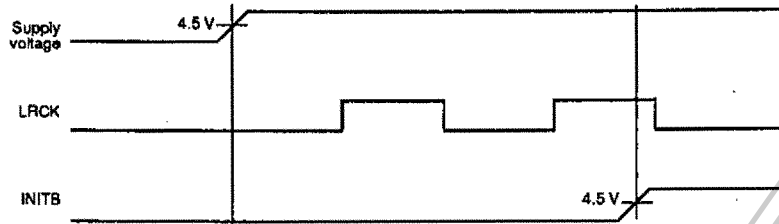
Figure 6. Initialization
