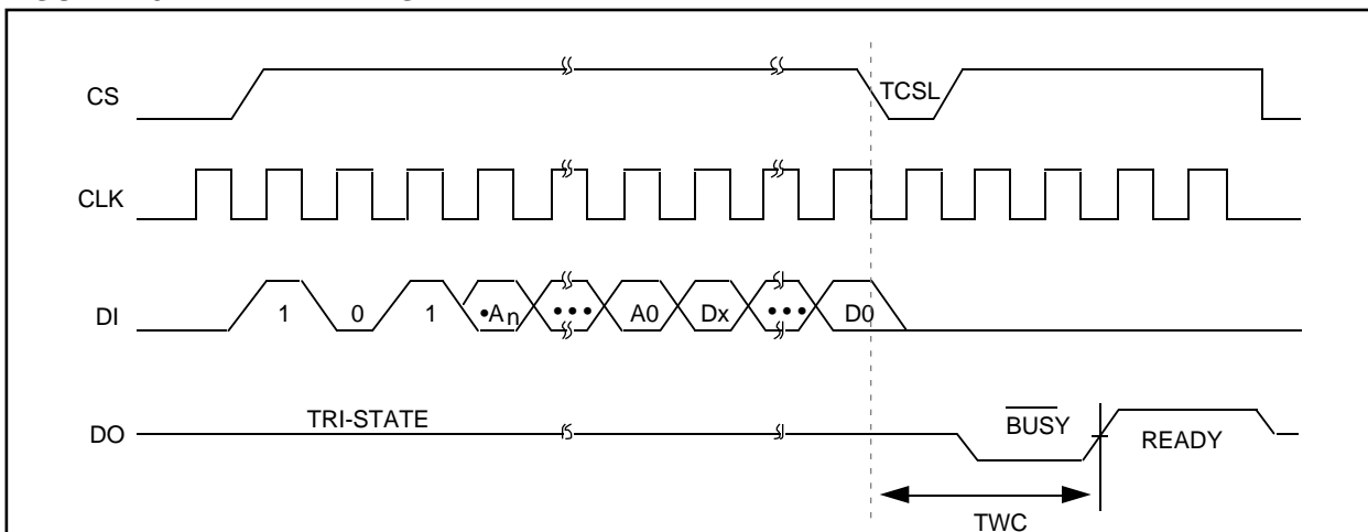
FIGURE 2-5: WRITE TIMING
