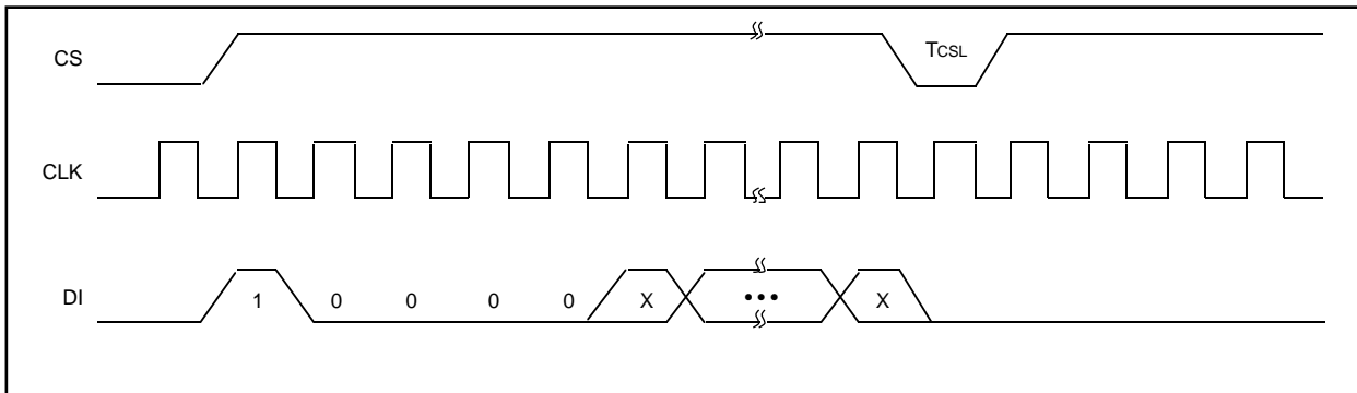
FIGURE 2-5: WRITE TIMING
