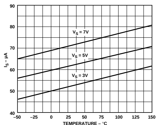
Figure 5. Supply Current vs. Temperature ( V_{OUT} = HIGH )
