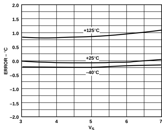
Figure 7. Setpoint Error vs. Supply Voltage
