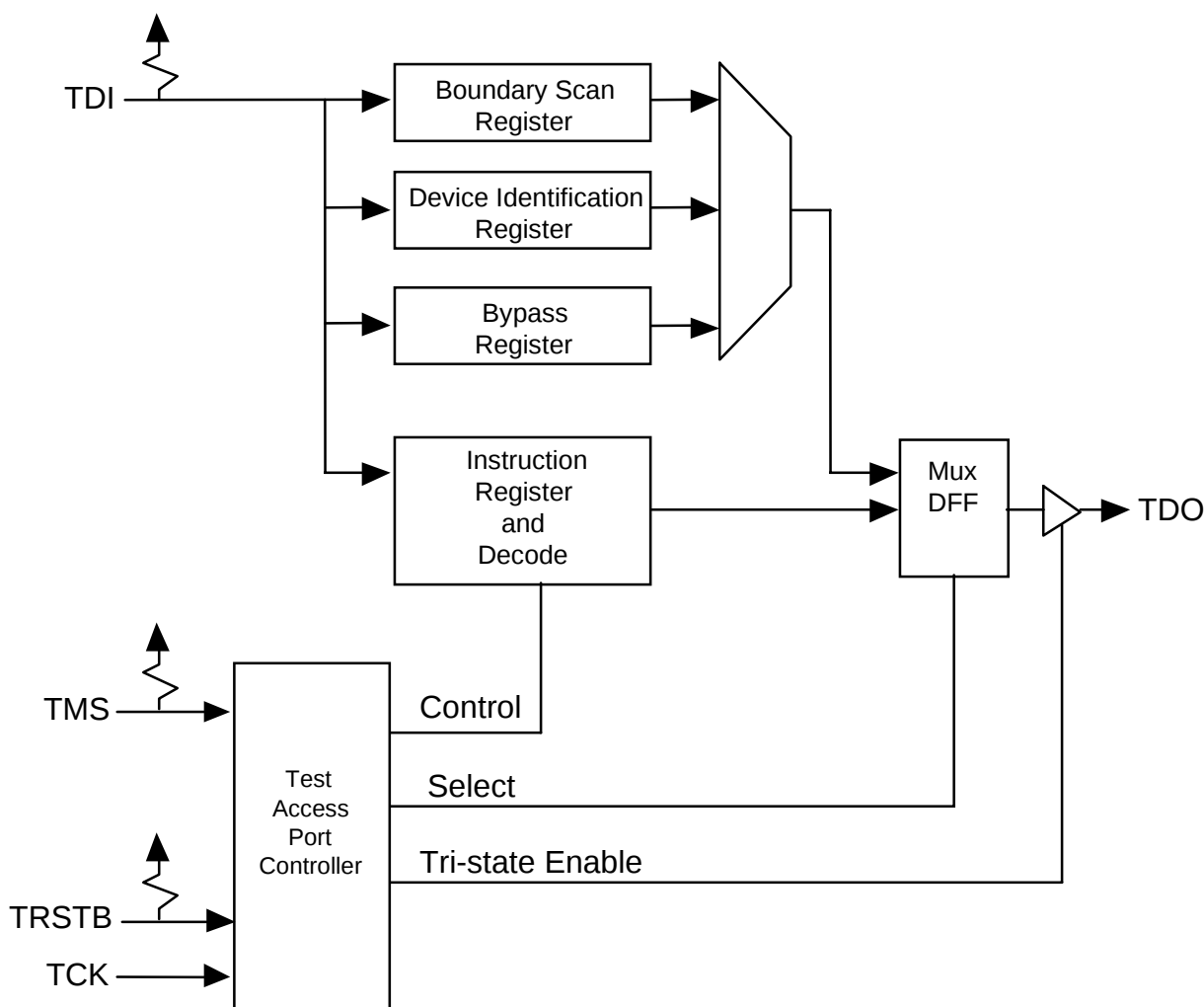
Figure 37 Boundary Scan Architecture
