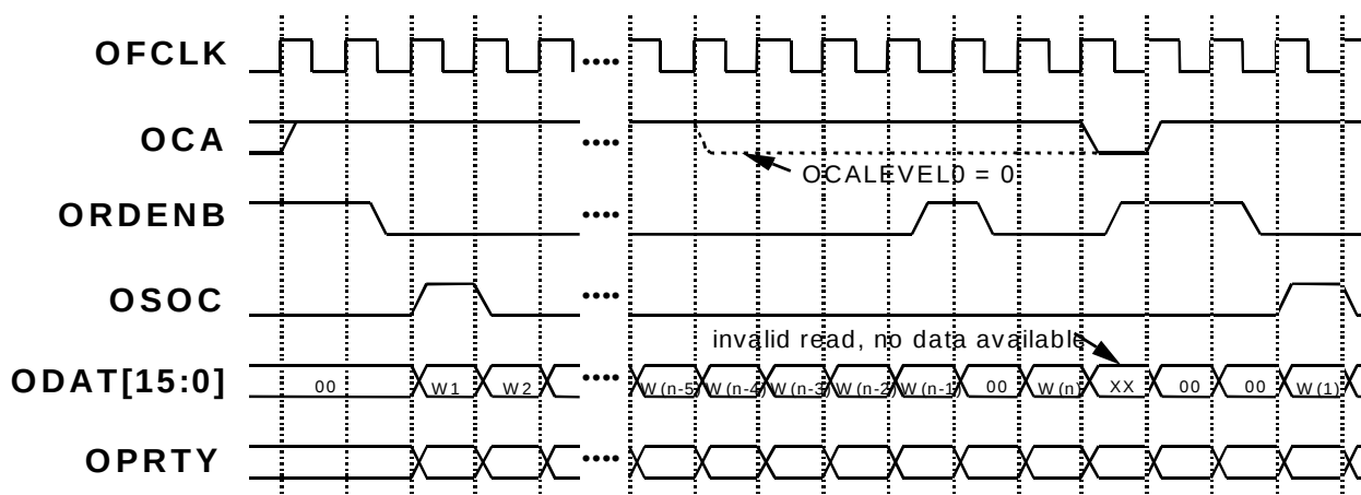
Figure 42 Ingress Output Cell Interface (OTSEN=0)
