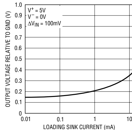
Output Low Voltage vs Sink Current
