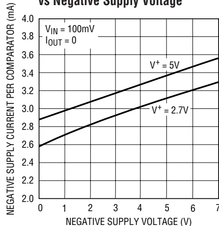
Negative Supply Current vs Negative Supply Voltage
