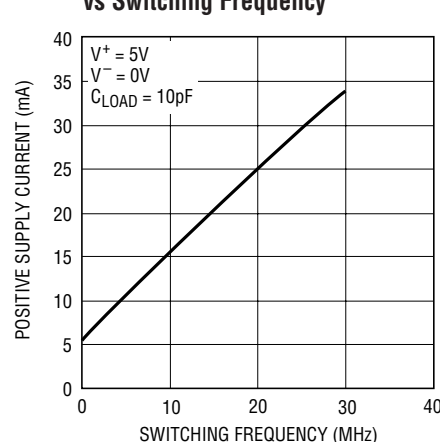
Positive Supply Current vs Switching Frequency
