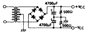
Specified Transformer Power Supply (Equivalent to RP-25)
