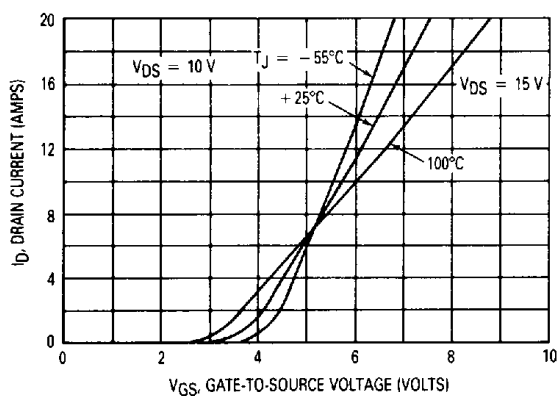
Figure 4. Transfer Characteristics
