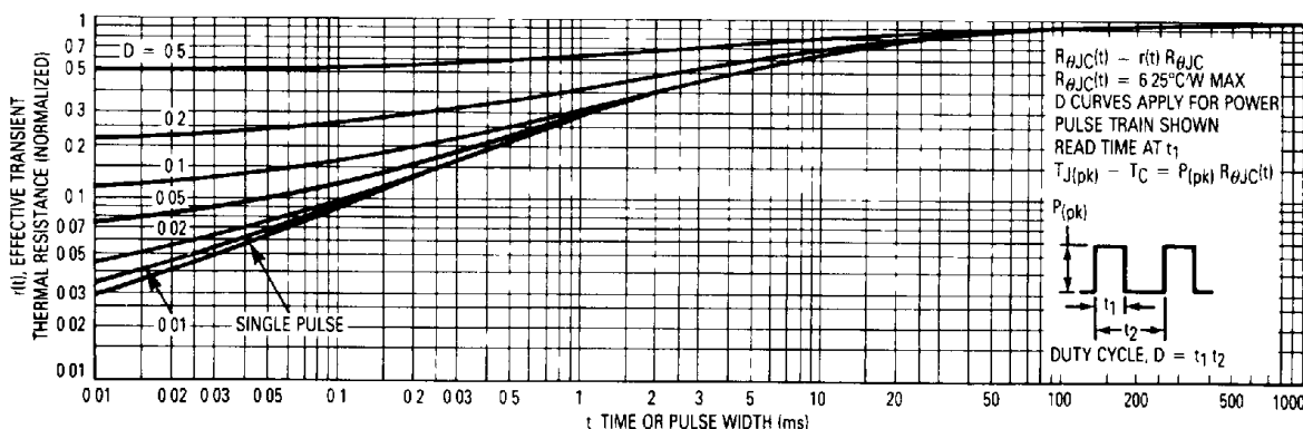
Figure 10. Thermal Response
