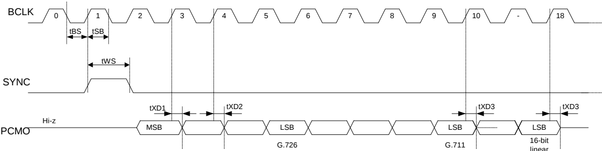
Fig. 5 PCM I/F mode output timing (short frame)
