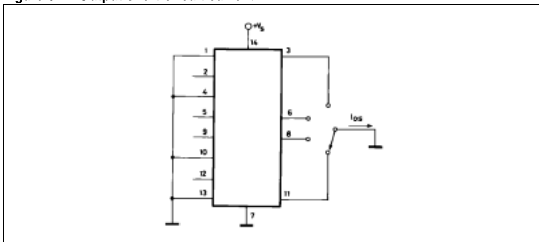
Figure 6. Output short-circuit current
