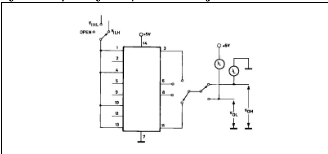
Figure 7. Output voltage and input threshold voltage
