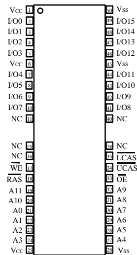
44(50) TSOP II
