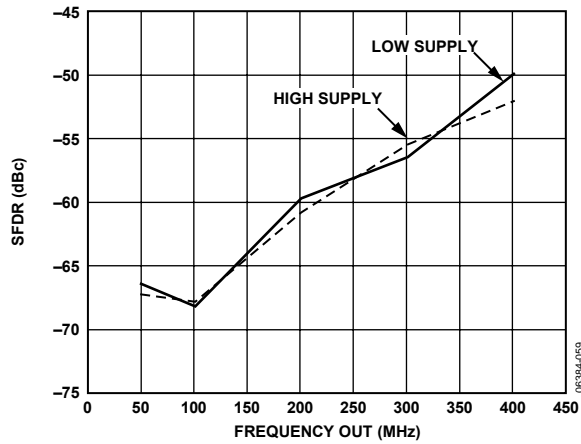
Figure 18. SFDR vs. Output Frequency vs. Supply ( \pm 5\% ) in Single Tone Mode
