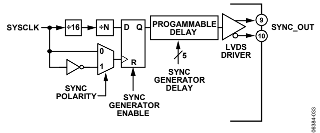
Figure 55. Sync Generator
