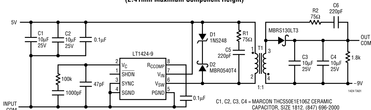
-9V PCMCIA Type II Isolated LAN Supply (2.41mm Maximum Component Height)
