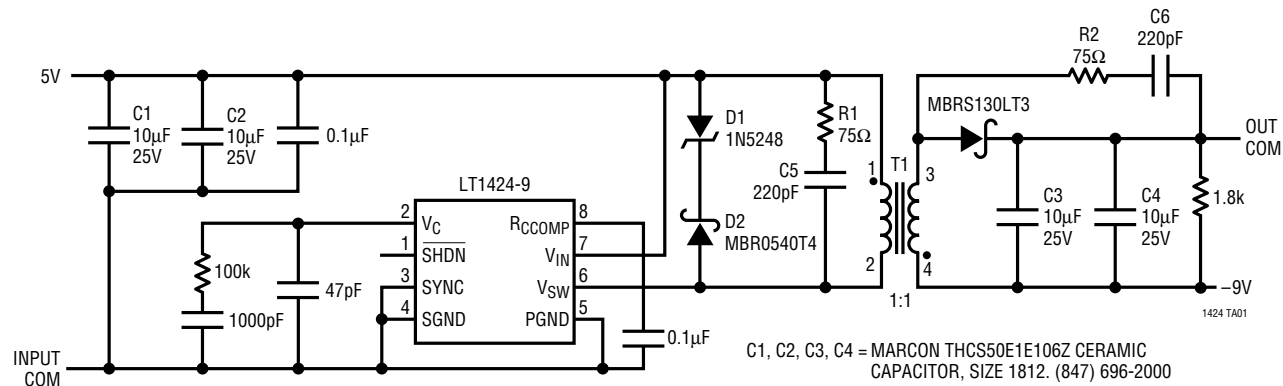
-9V PCMCIA Type II Isolated LAN Supply
