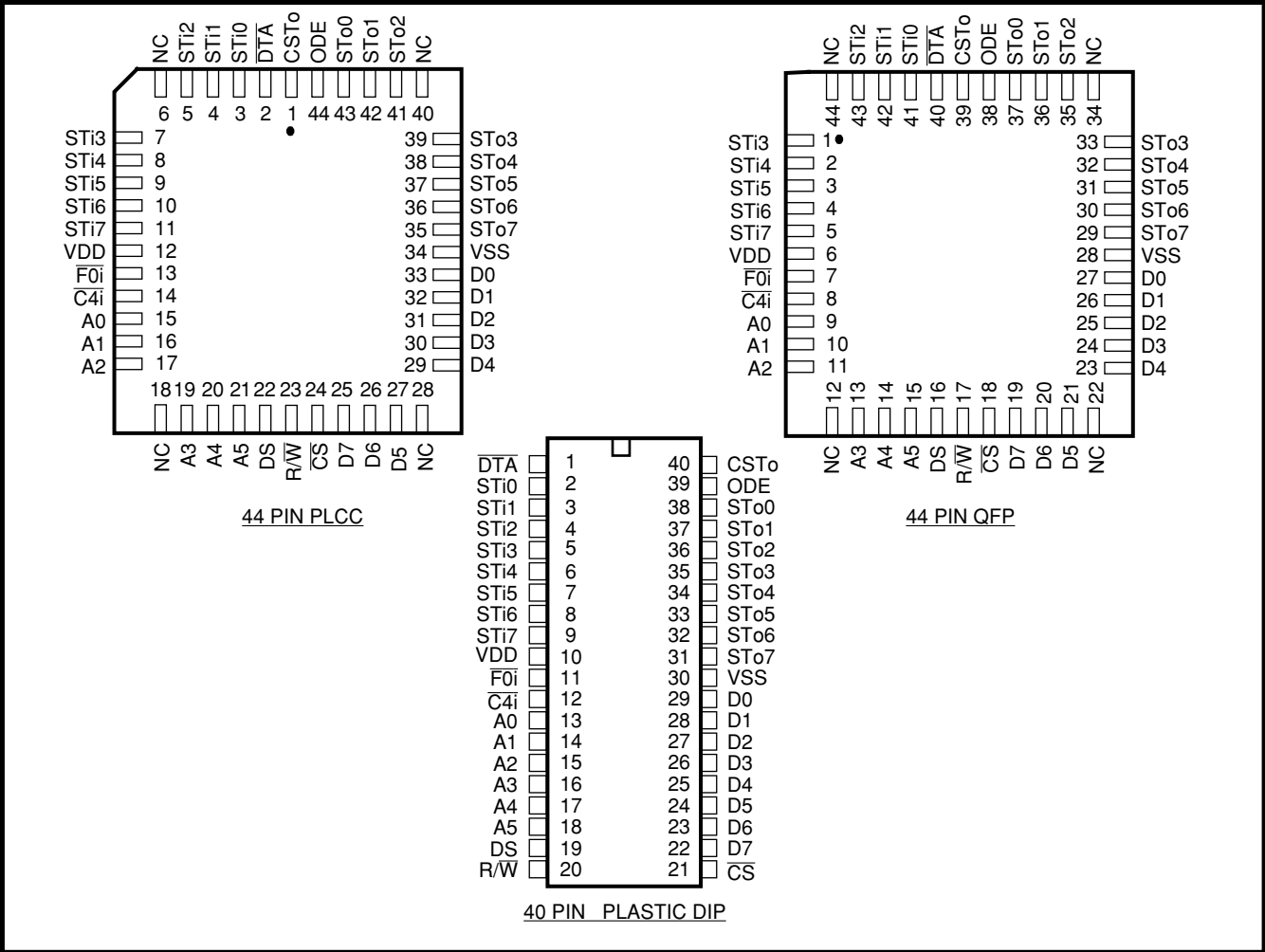
Figure 2 - Pin Connections
