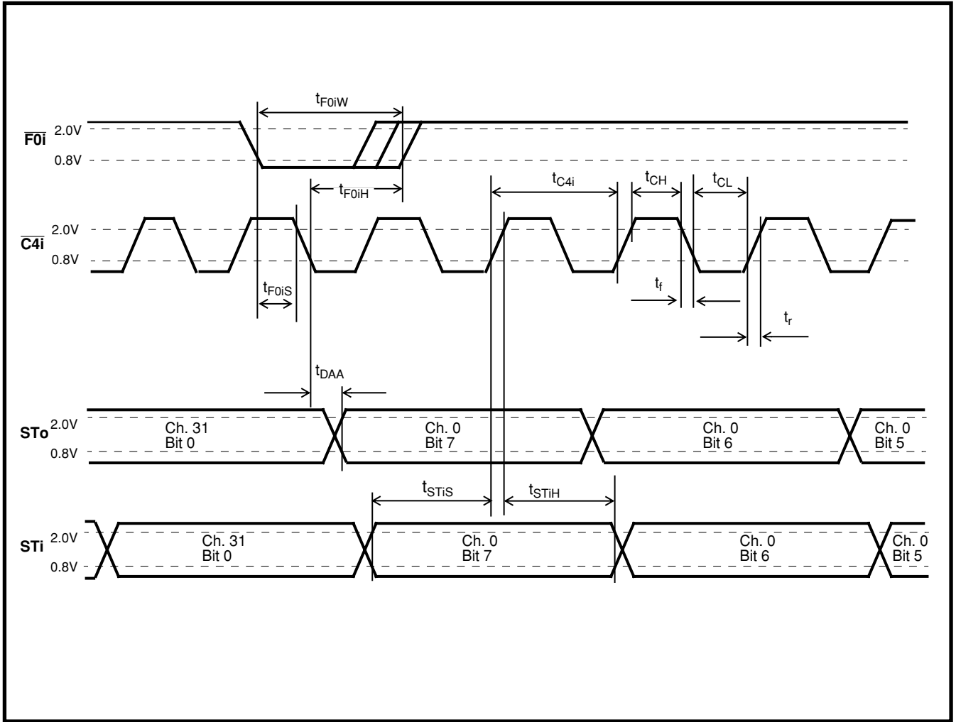
Figure 13 - ST-BUS Timing
