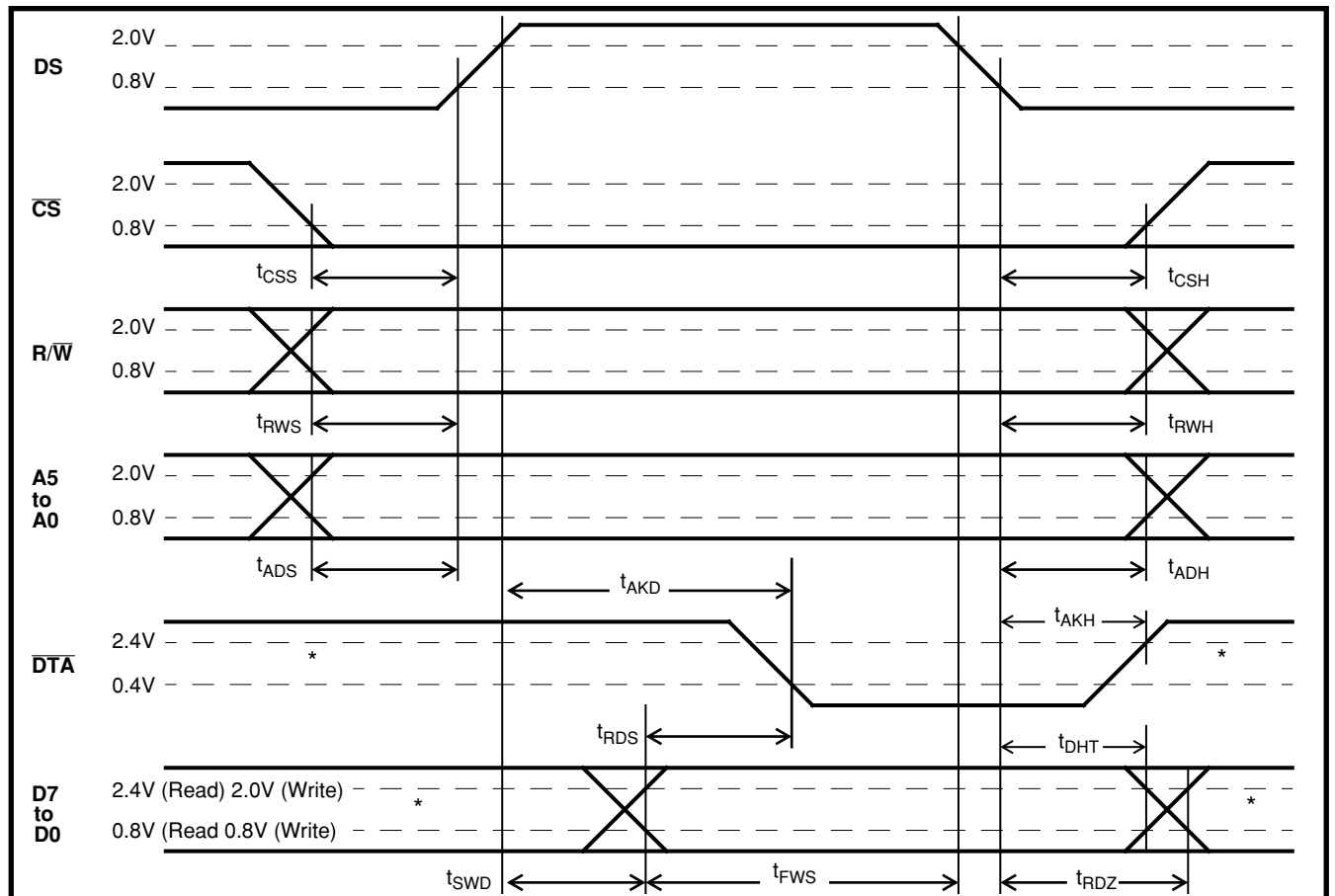
Figure 17 - Processor Bus
