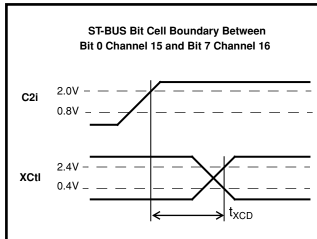
Figure 16 - XcTi Timing
