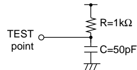
Figure 5 Timing Load
