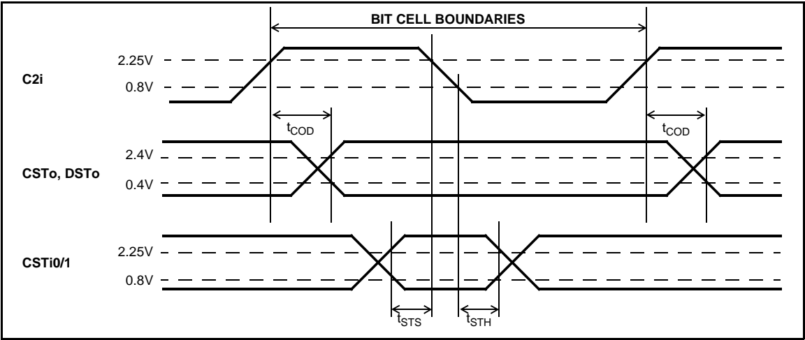
Figure 13 - ST-BUS Timing - CSTo/DSTo Altered by PMAC
