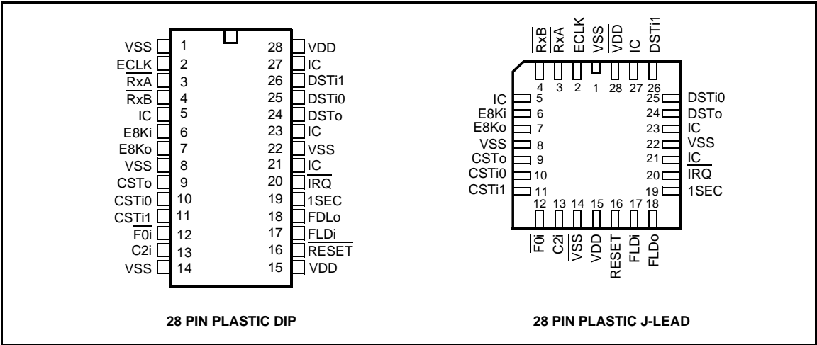
Figure 2 - Pin Connections
