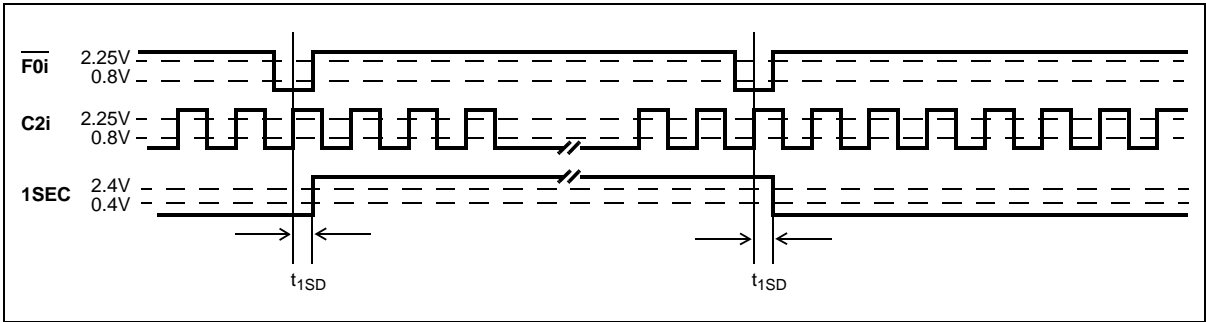
Figure 16 - 1SEC Timing
