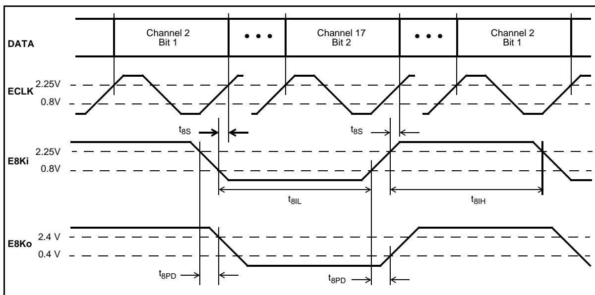
Figure 12 - 8kHz Extracted Framing Signal
