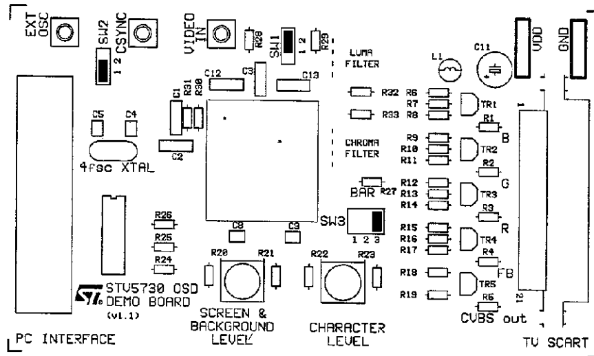
Figure 2 : STV5730 Evaluation Board Diagram
