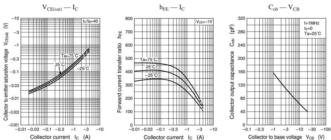
Characteristics charts of NPN transistor block
