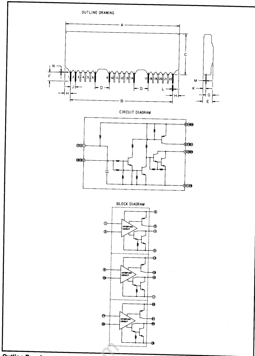
Outline Drawing
