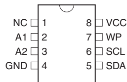
8-lead TSSOP
