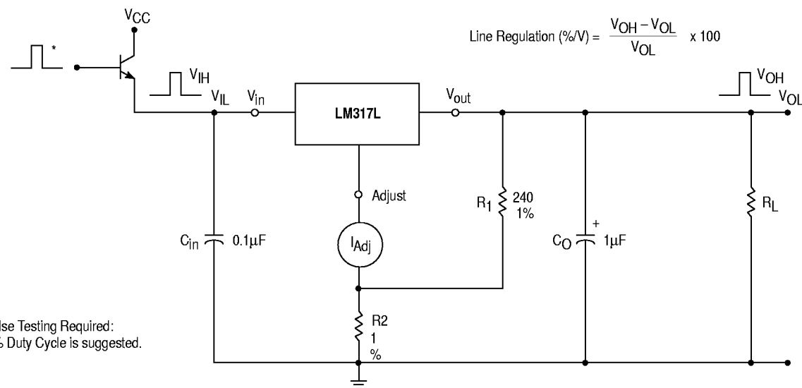
Figure 1. Line Regulation and \Delta I_{Adj}/Line Test Circuit
