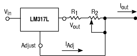
Figure 22. Current Regulator
