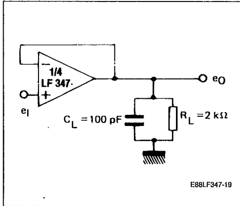
Figure 1 : Voltage Follower.
