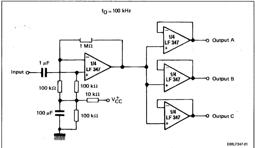
Figure 3 : Voltage Follower.
