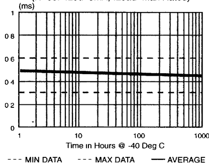
58) ILED Stability
