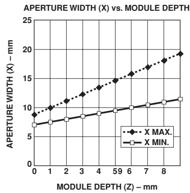
Figure 20. Aperture width (X) vs. module depth.
