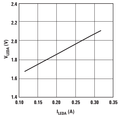
Figure 10. V_{LED} vs I_{LED} .
