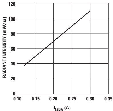
Figure 9. Radiant Intensity vs I_{LED} .
