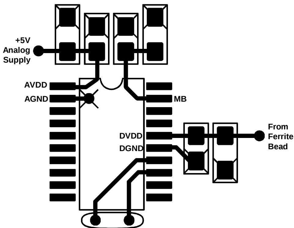
Figure 6. Suggested Layout
