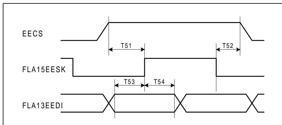
Figure 31. EEPROM Timings
