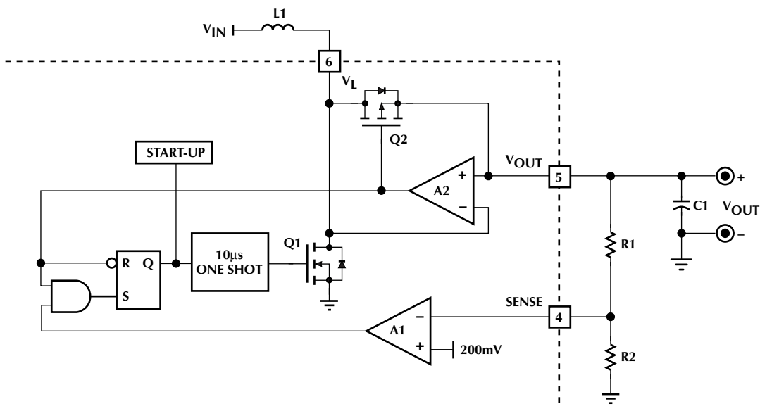
Figure 2. PFM Regulator Block Diagram.
