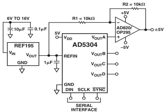
Figure 15. Bipolar Operation with the AD5304
