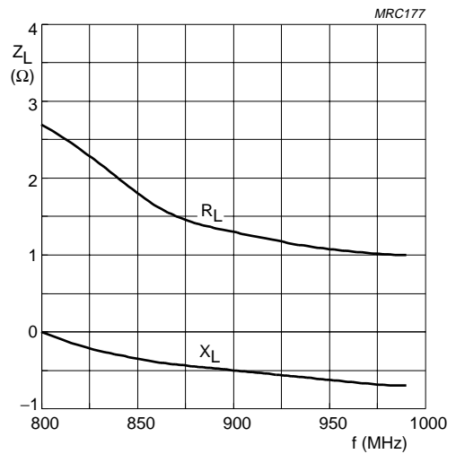
Fig.11 Load impedance; series components; V_{CE} = 24\text{ V} ; P_L = 35\text{ W} ; R_{th\text{ mb-h}} = 0.4\text{ K/W} ; typical values.
