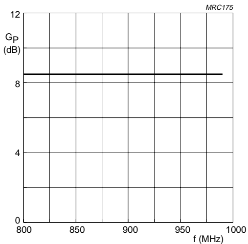
Fig.12 Power gain; class-AB operation; V_{CE} = 24\text{ V} ; P_L = 35\text{ W} ; R_{th\text{ mb-h}} = 0.4\text{ K/W} ; typical values.
