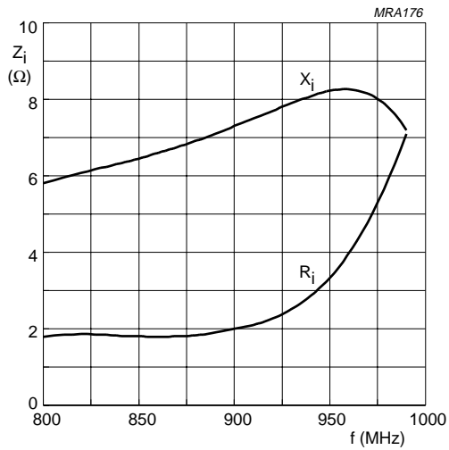
Fig.10 Input impedance; series components; V_{CE} = 24\text{ V} ; P_L = 35\text{ W} ; R_{th\text{ mb-h}} = 0.4\text{ K/W} ; typical values.
