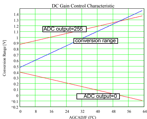
Fig. 2-18: Fast-blank ADC characteristic without clamping ( DCLMPF=1 )
