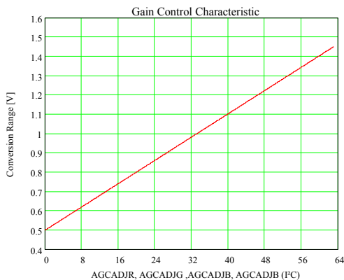
Fig. 2-17: RGBF ADC characteristic
