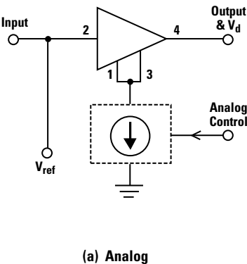
Figure 6. Adaptive Bias Control.
