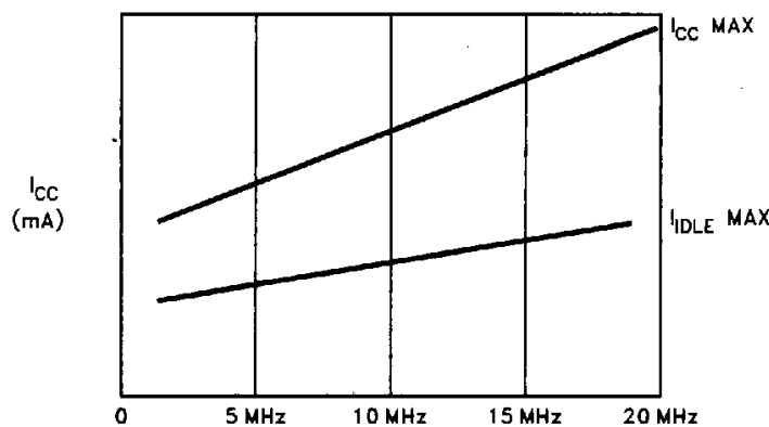
I_{CC} vs Frequency
