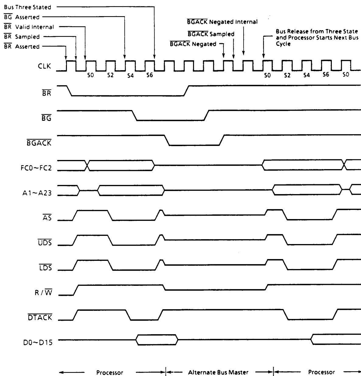
Figure 4.17 Bus Arbitration Timing Diagram – Special Case
