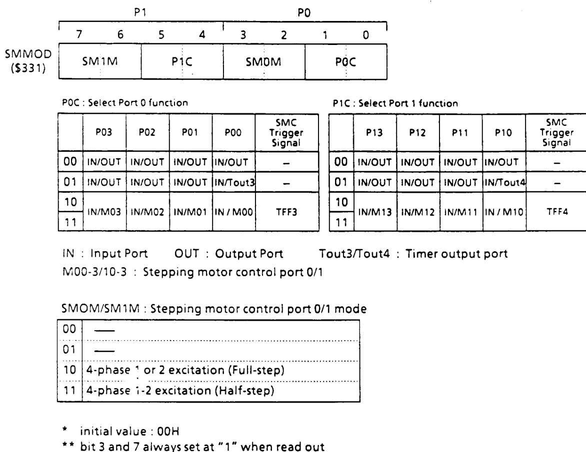
Figure 6.36 Register for Port 0 and 1
