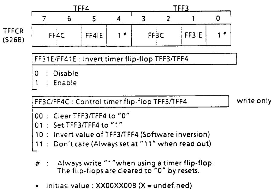
Figure 6.53 8-bit Timer Flip-flop Control Register (TFFCR)
