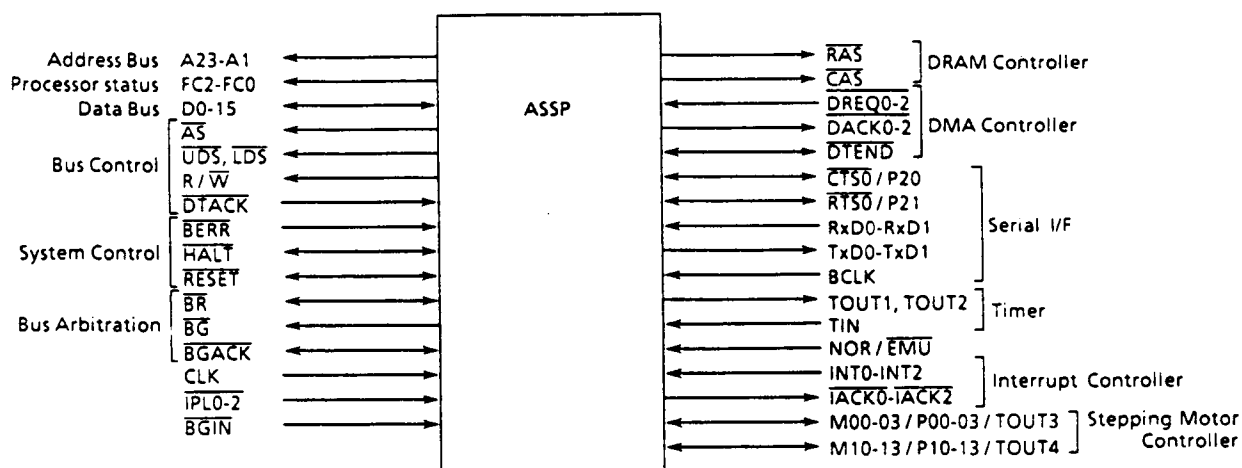
Figure 4.2 Normal Mode Signals Input/Output as Bus Master
