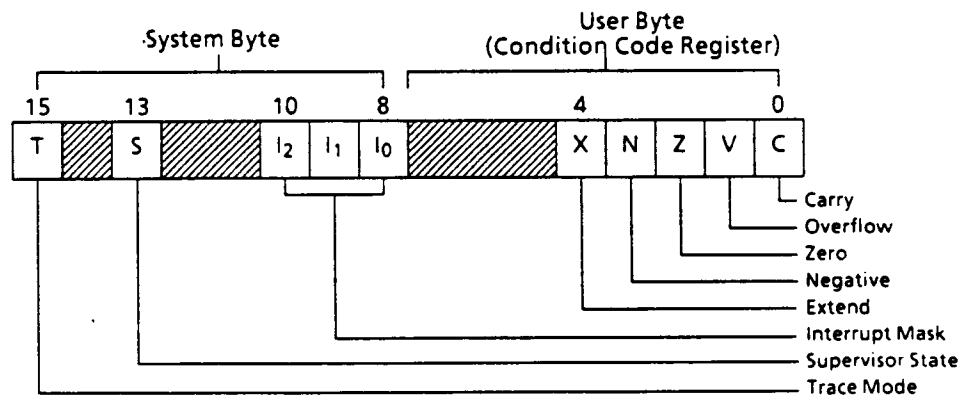
Figure 1.4 Status Register
