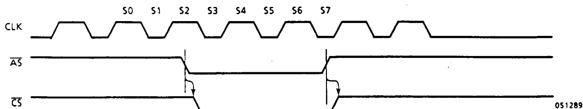
Figure 6.1 \overline{CS} and \overline{AS}
