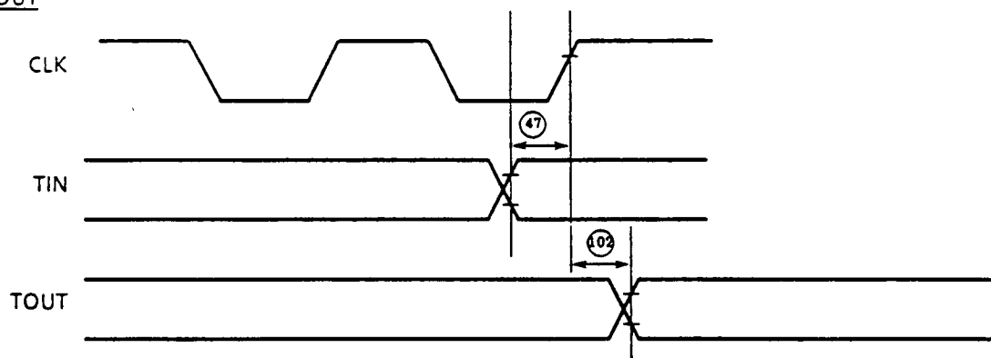
Figure 8.7 Timer Input / Output Timing
