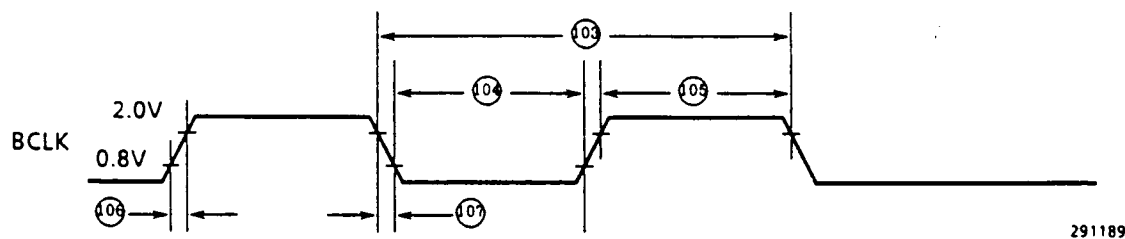
Figure 8.8 Baud Rate Clock Timing
