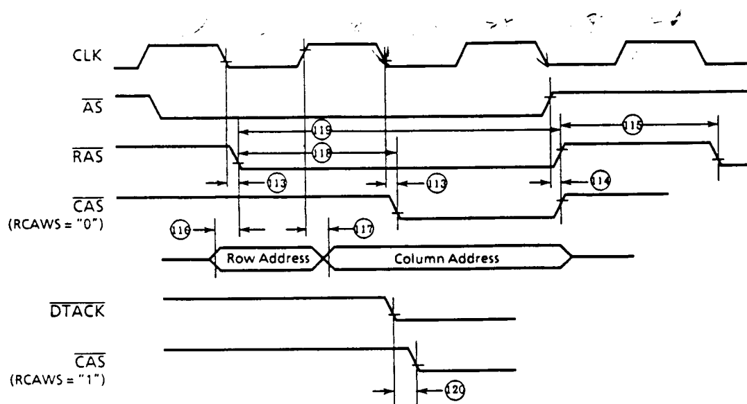
Figure 8.10 DRAM Read / Write
