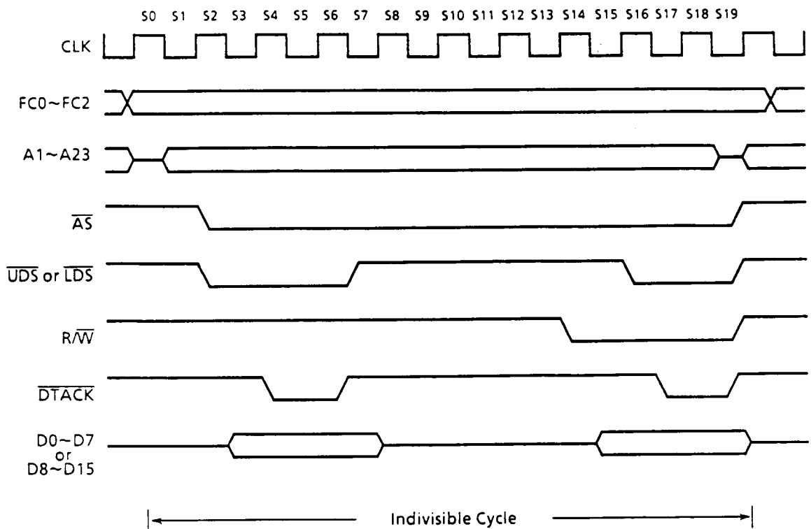
Figure 4.10 Read-Modify-Write Cycle Timing Diagram
