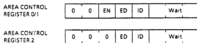
Figure 6.6 Area Control Register
