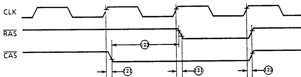
Figure 8.11 DRAM Refresh
