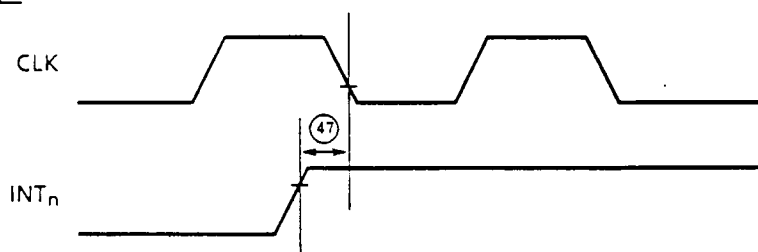
Figure 8.6 Interrupt Request Timing
