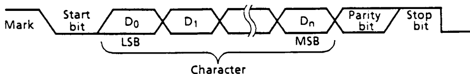
Figure 6.22 Data Frame Sequence
