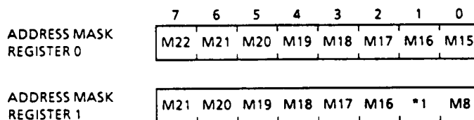
Figure 6.5 Address Mask Register
