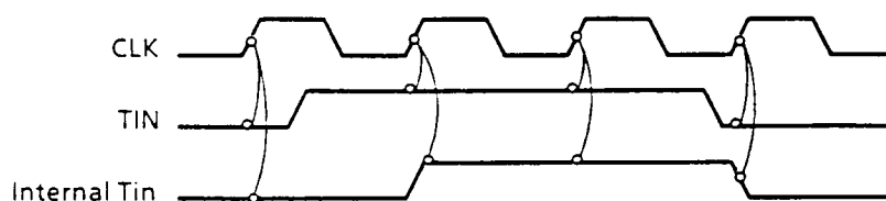
Figure 6.41 TIN Timing
