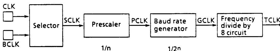
Figure 6.24 Baud Rate Generator Block
