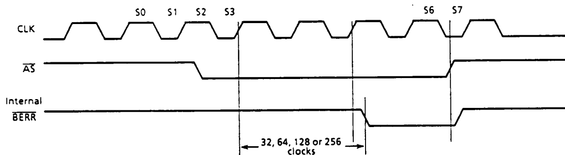
Figure 6.3 Internal \overline{BERR}
