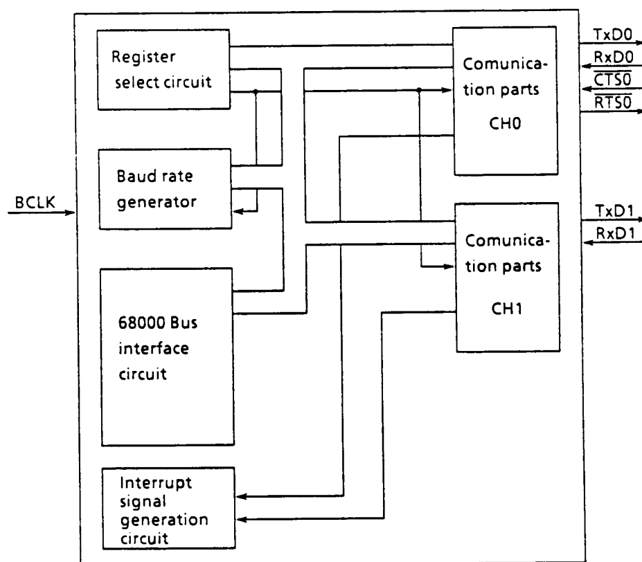
Figure 6.19 Serial Interface Block Diagram
