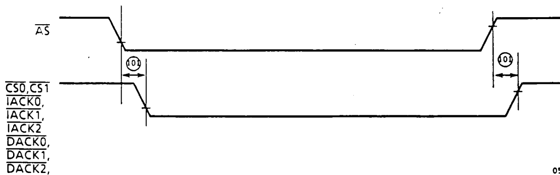
Figure 8.5 \overline{CS}, \overline{IACK} Timing
