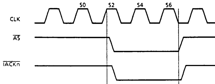
Figure 6.11 IACK signal
