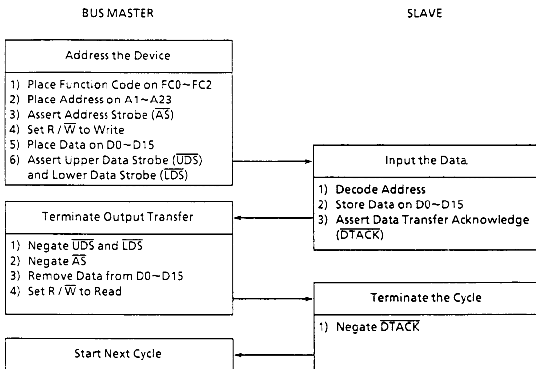
Figure 4.6 Word Write Cycle Flowchart
