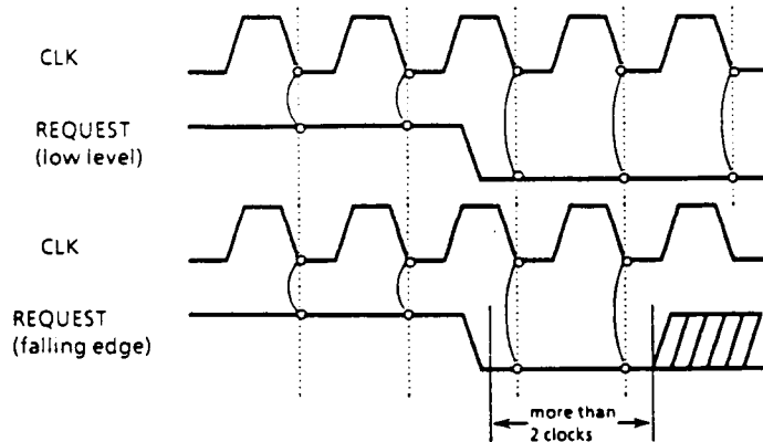
Figure 6.10 Interrupt request
