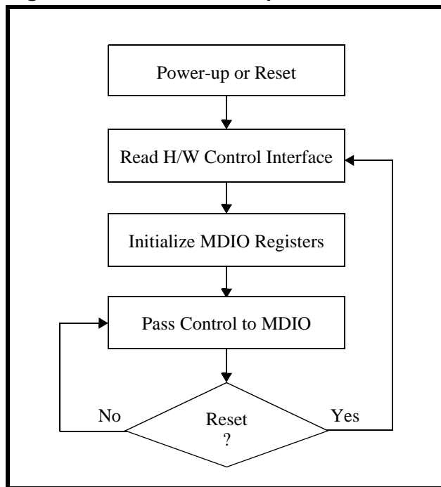
Figure 7: Initialization Sequence
