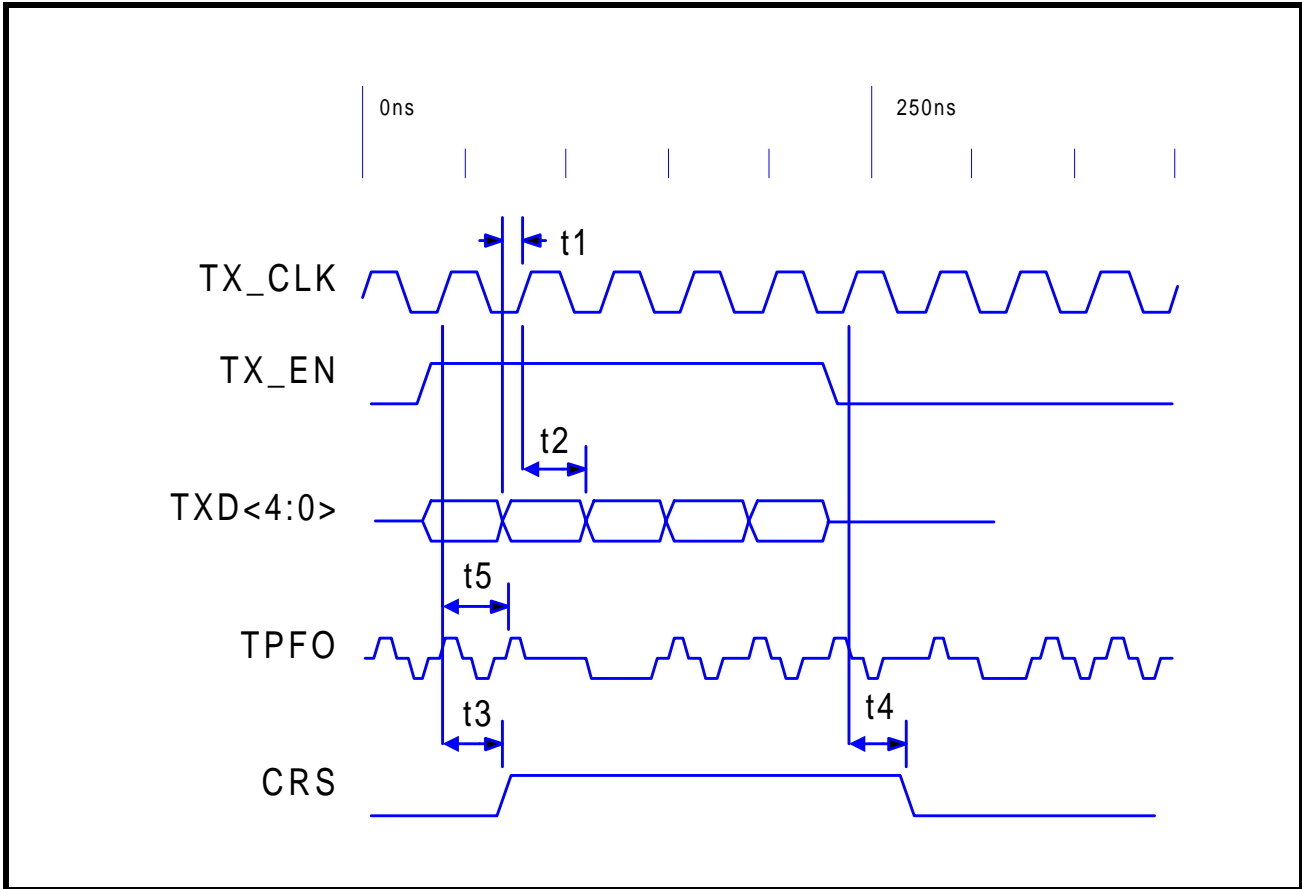
Figure 22: 100BASE-TX Transmit Timing (5B Mode)
