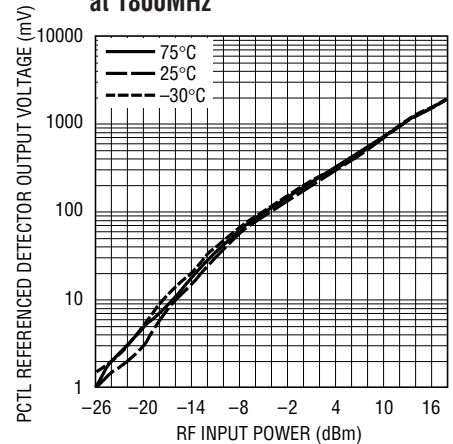
LTC4400-2 Detector Characteristics at 1800MHz
