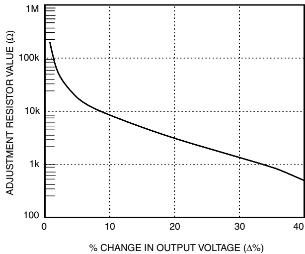
Figure 17. Resistor Selection for Decreased Output Voltage
