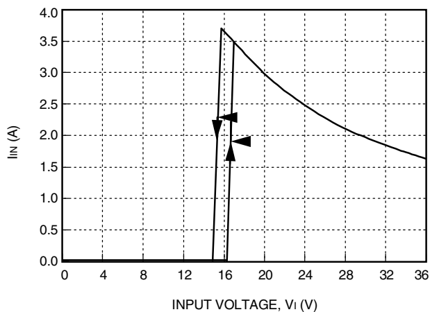
Figure 1. Typical JC050B Input Characteristics at Room Temperature, I_o = Full Load
