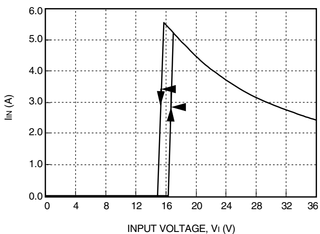
Figure 2. Typical JC075B Input Characteristics at Room Temperature, I_o = Full Load
