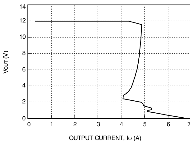
Figure 4. Typical JC050B Output Characteristics at Room Temperature, V_{IN} = 28 V
