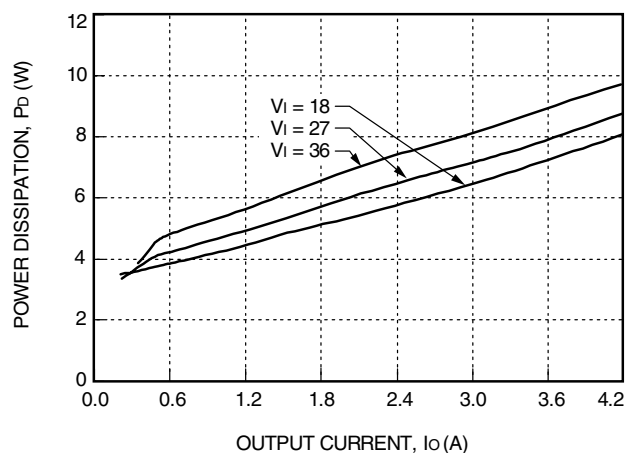
Figure 22. JC050B Power Dissipation vs. Output Current
