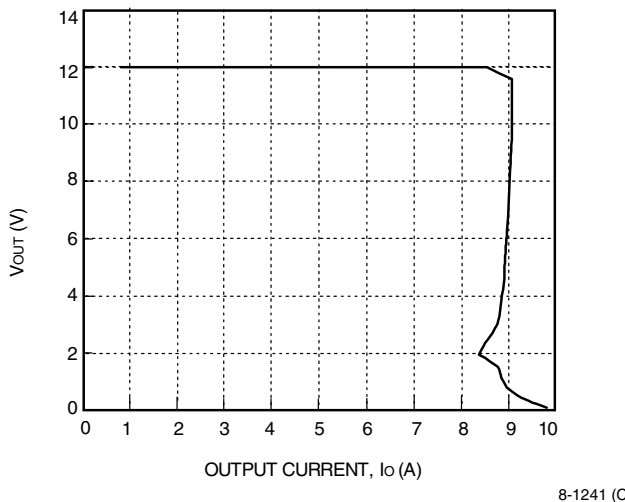
Figure 6. Typical JC100B Output Characteristics at Room Temperature, V_{IN} = 28\text{ V}
