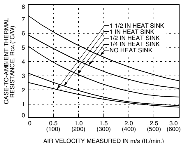
Figure 25. Case-to-Ambient Thermal Resistance Curves; Either Orientation
