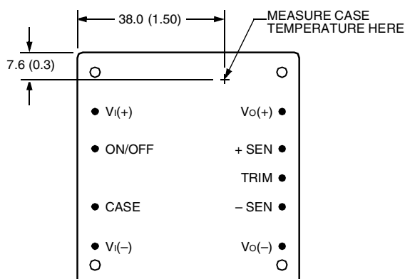
Figure 20. Case Temperature Measurement Location
