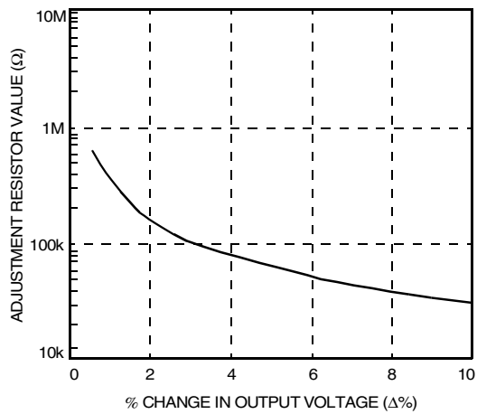
Figure 19. Resistor Selection for Increased Output Voltage
