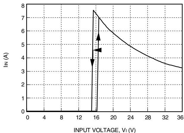
Figure 3. Typical JC100B Input Characteristics at Room Temperature, I_o = Full Load
