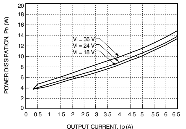
Figure 23. JC075B Power Dissipation vs. Output Current
