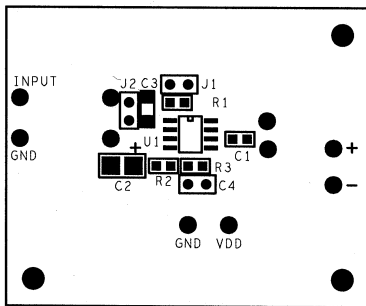
Silk Screen
