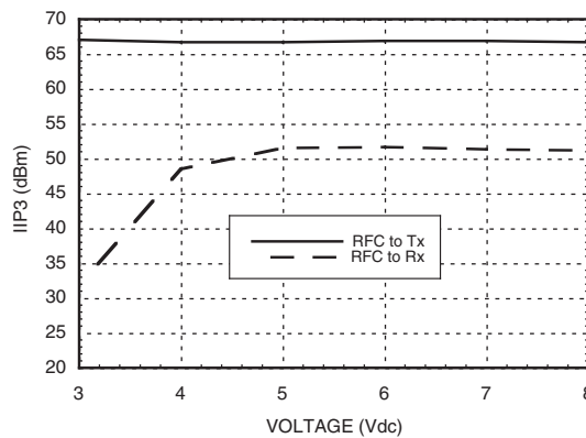
Input IP3 vs. Voltage with 457 MHz Tuning
