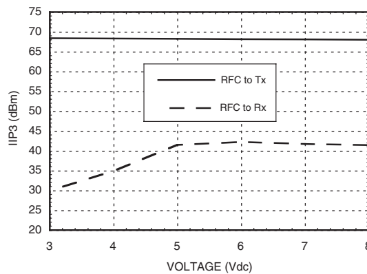
Input IP3 vs. Voltage with 1843 MHz Tuning
