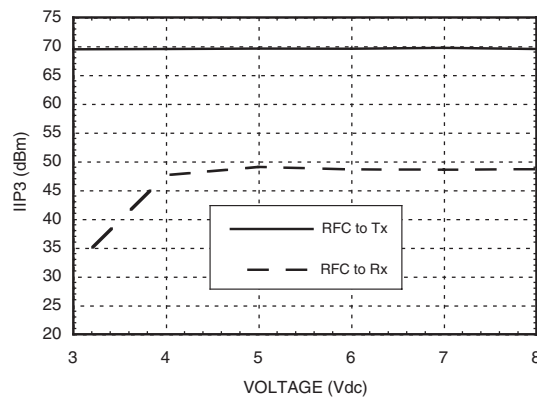
Input IP3 vs. Voltage with 785 MHz Tuning
