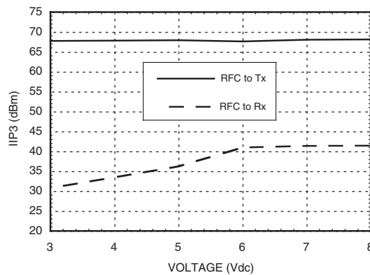
Input IP3 vs. Voltage with 1960 MHz Tuning
