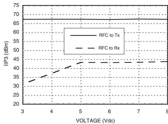
Input IP3 vs. Voltage with 2140 MHz Tuning
