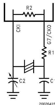
FIGURE 10. Crystal Oscillator
