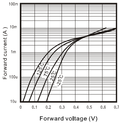
Fig. 1 - Forward characteristics
