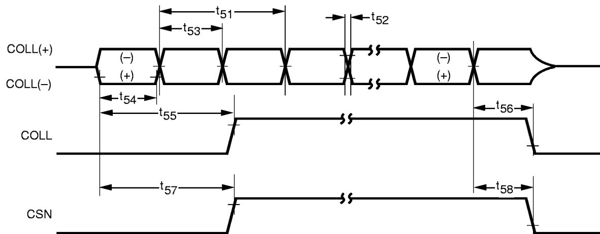
Figure 11. Collision Timing
