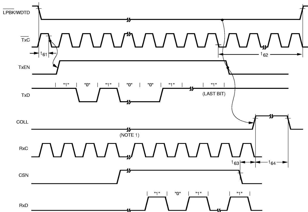
Figure 13. Loopback Timing
